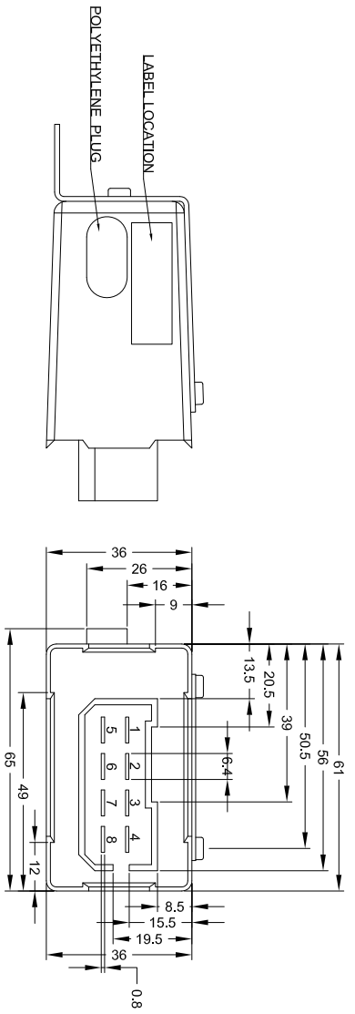
MATING CONNECTOR DETAIL
